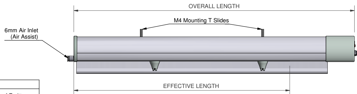
971IPS 30kV Standard Lengths
